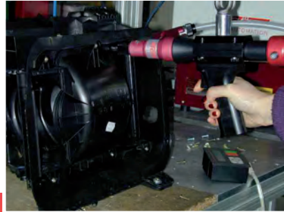
Horizontal assembly of air-conditioner units
