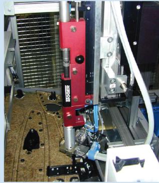
Assembling motor vehicle door trim panel
