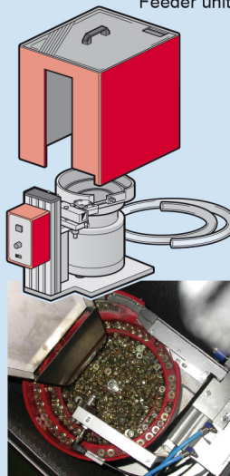
Feeder unit
